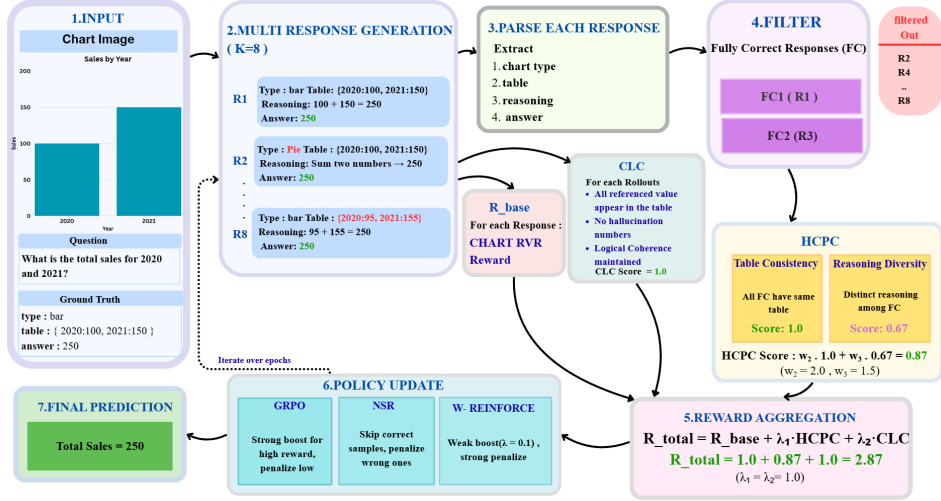
Figure 3.1: Overview of the HCPC-RLVR training pipeline. A chart image and question enter the system; the proposed model generates K = 8 rollouts; each rollout is parsed into chart type, table, reasoning, and answer; the fully-correct subset feeds HCPC; and the aggregated reward drives the policy update. Current experiments use K = 4 rollouts because of compute constraints.
